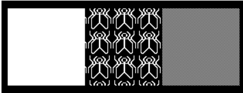
Figure 2-11 Stippled Polygons
