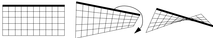
Figure 2-4 Nonplanar Polygon Transformed to Nonsimple Polygon
